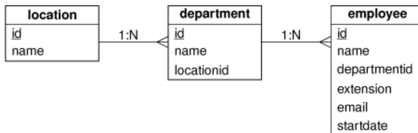
Figure 13.2. The Staff Manager application's tables
