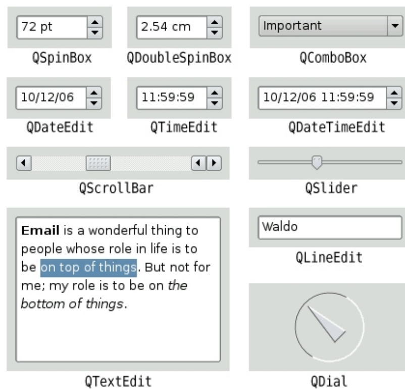
Figure 2.22. Qt's input widgets
