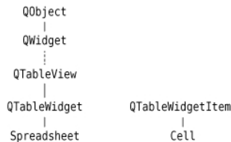
Figure 4.1. Inheritance trees for Spreadsheet and Cell
