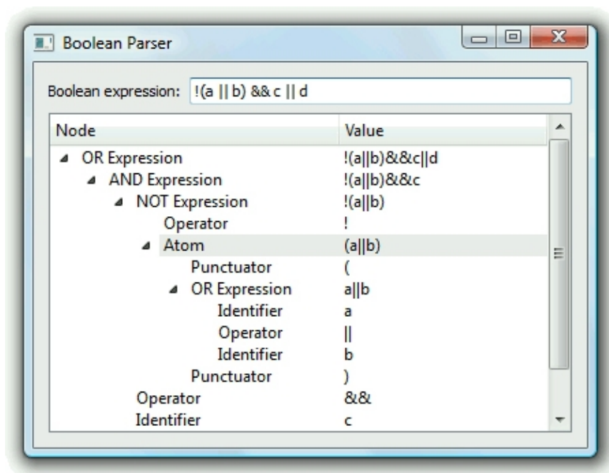
Figure 10.14. The Boolean Parser application
