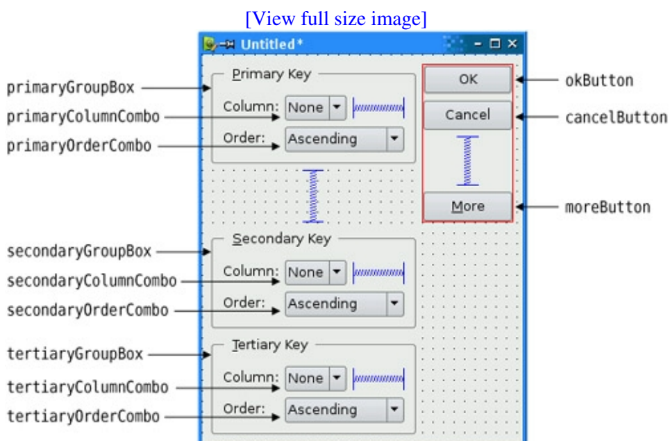
Figure 2.14. Naming the form's widgets
