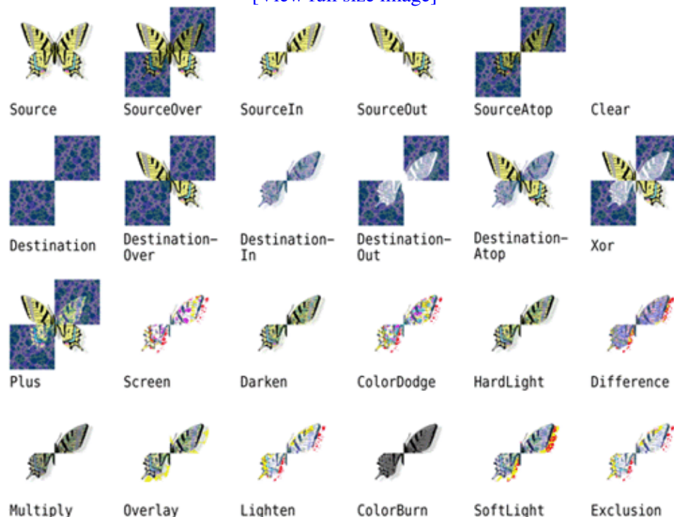
Figure 8.13. QPainter's composition modes
