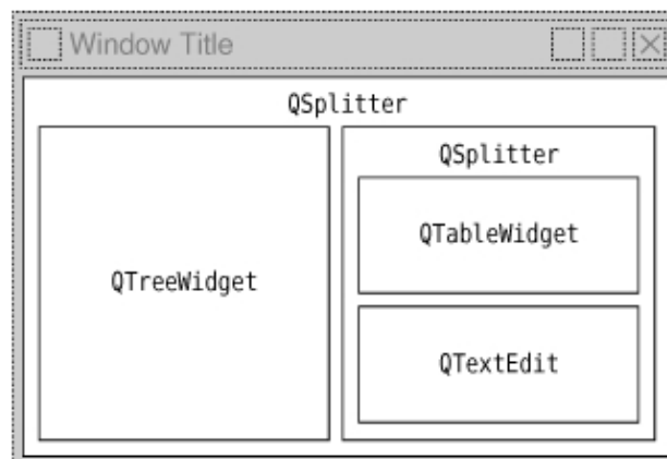
Figure 6.10. The Mail Client's splitter layout
