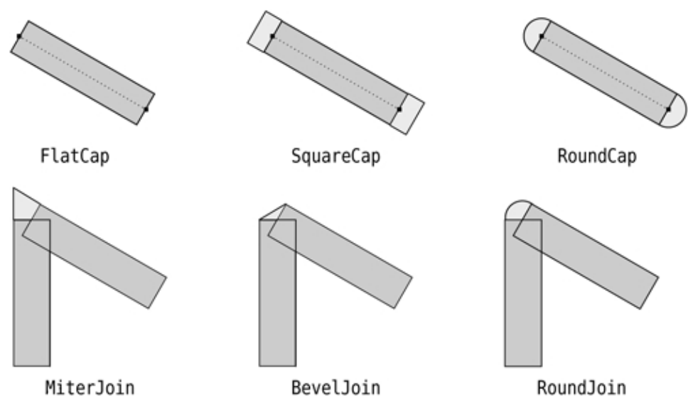
Figure 8.3. Line styles
