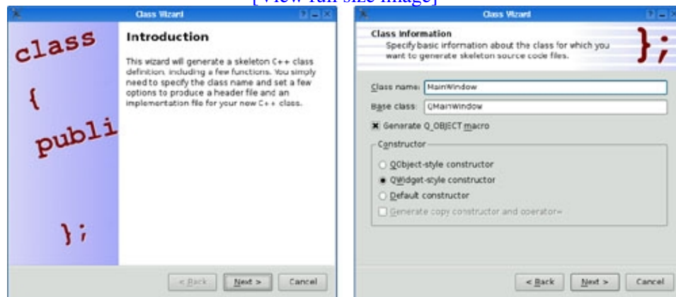
Figure 2.26. Qt's QWizard dialog
