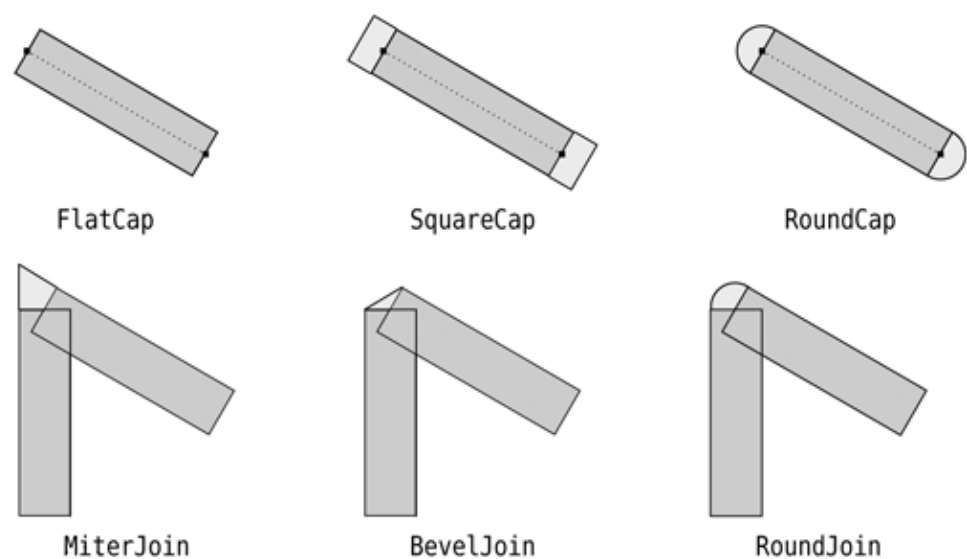
Figure 8.3. Line styles
