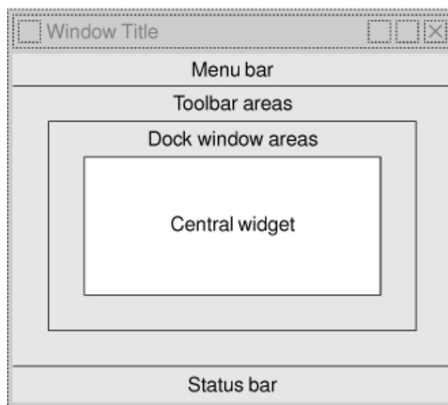
Figure 3.2. QMainWindow's areas
