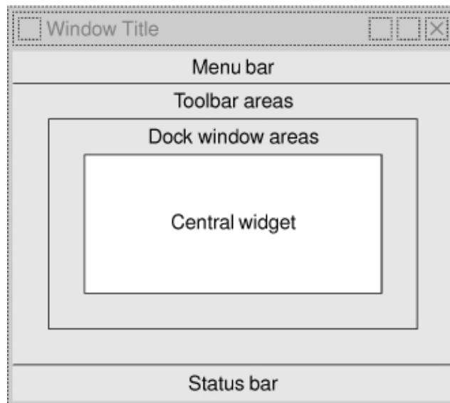
Figure 3.2. QMainWindow's areas
