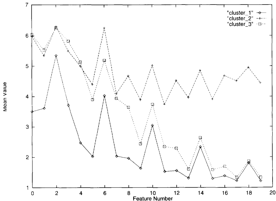
Fig. 12. Mean feature values of the 20 Gabor filters for the fingerprint image (Fig. 8). Cluster number 2 corresponds to the fingerprint regions in the image.
