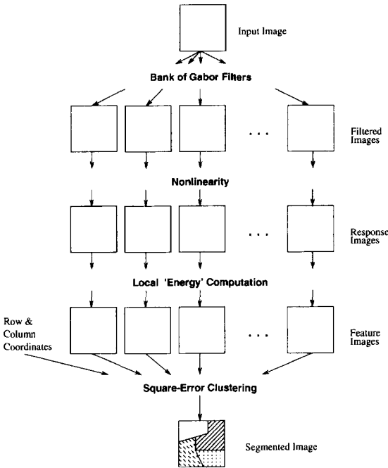
Fig. 1. An overview of the texture segmentation algorithm.
